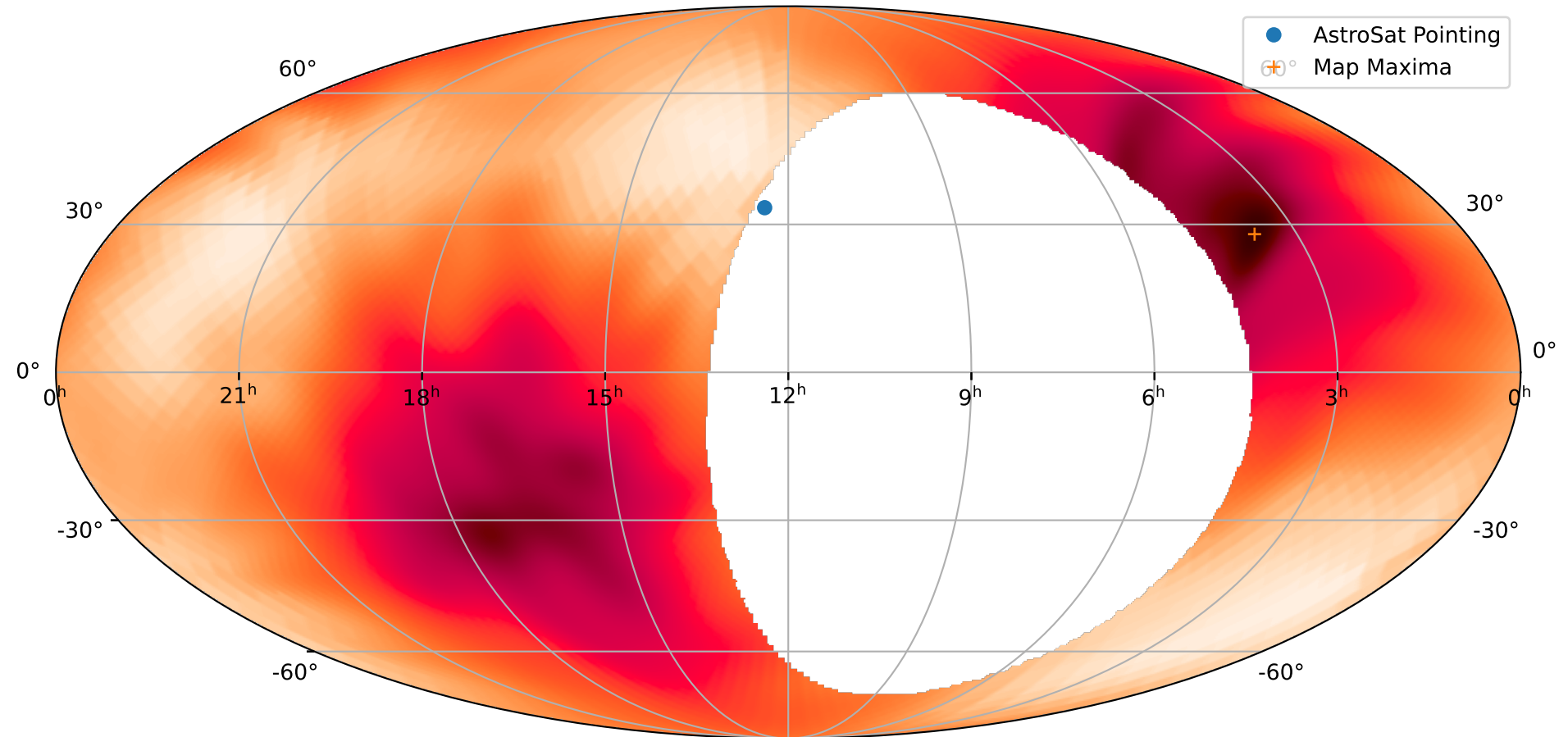
S230529ay as seen by AstroSat - (Prob covered: 76.0%)
