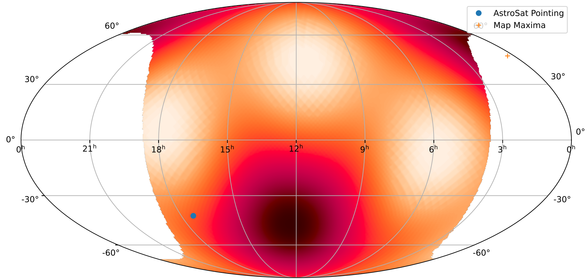
LVKN20230802T113359.000 as seen by AstroSat - (Prob covered: 70.0%)
