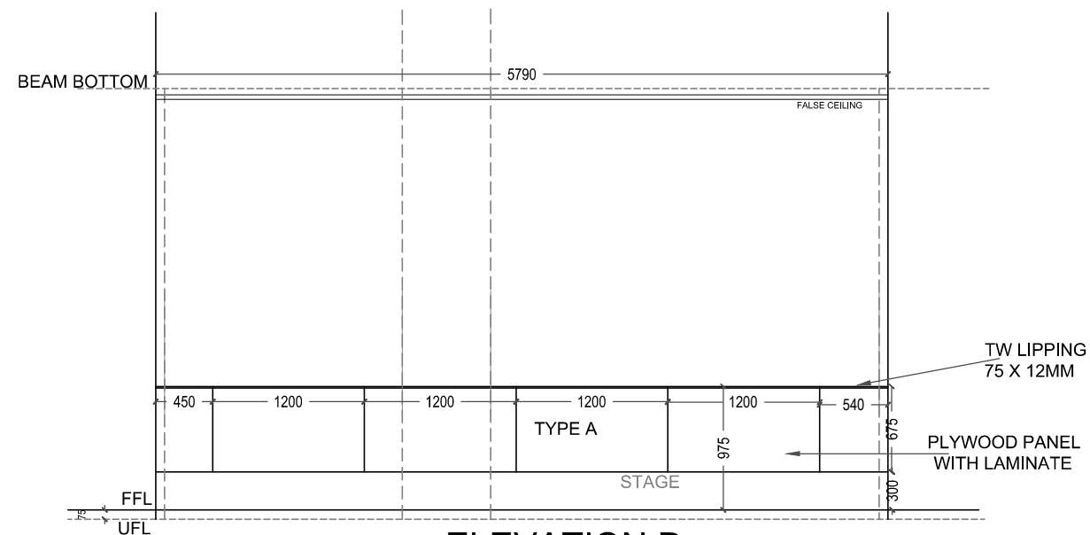
ELEVATION D
