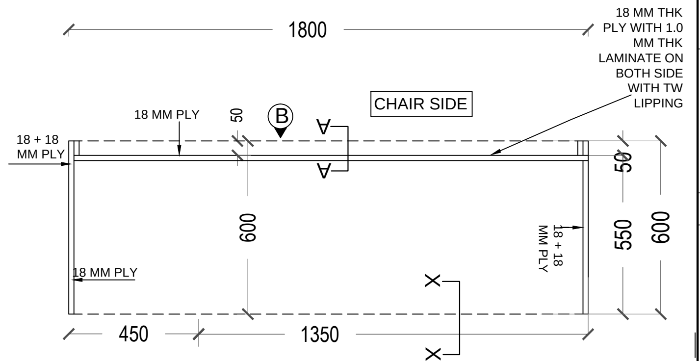
PLAN BELOW TABLE TOP
