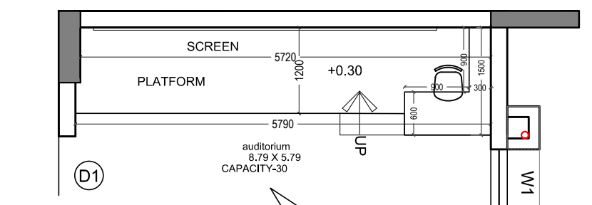
PLAN ABOVE TABLE TOP
