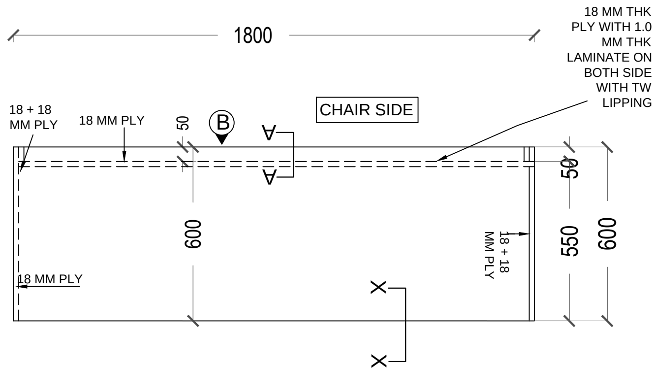
PLAN ABOVE TABLE TOP
