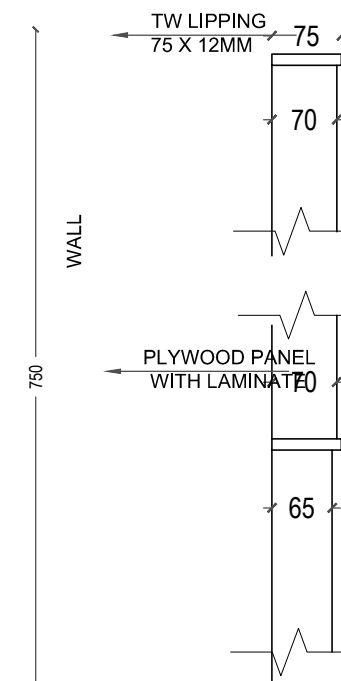
TYPICAL SECTION OF TYPE A PANEL
