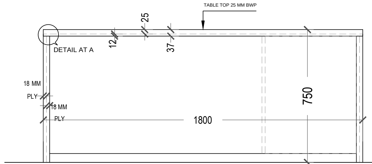
ELEVATION AT B
