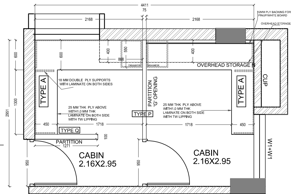
ROOM 4 - CABIN
