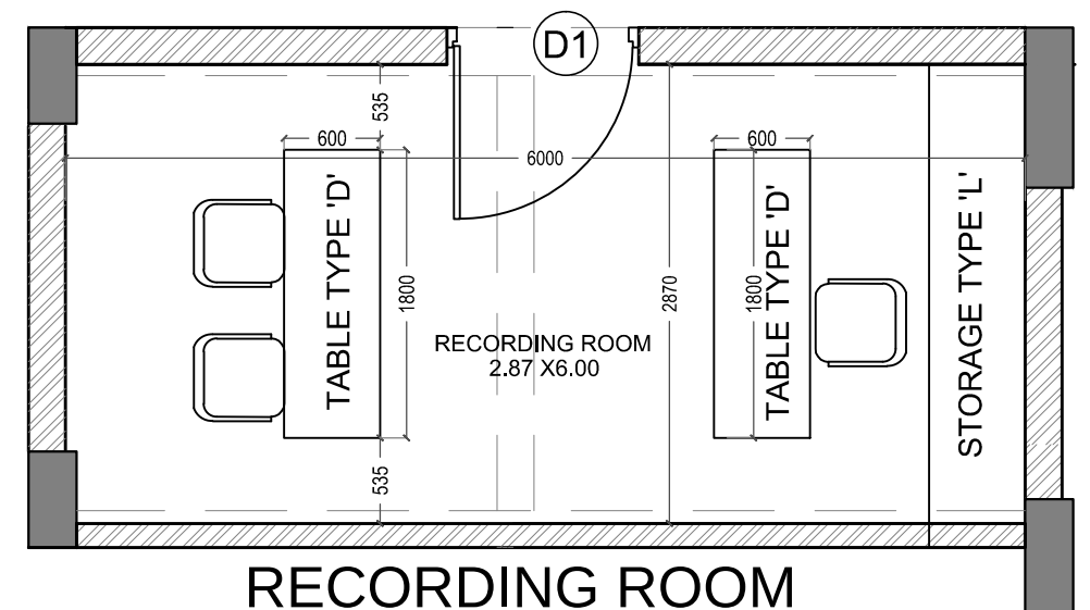
PLAN BELOW TABLE TOP
