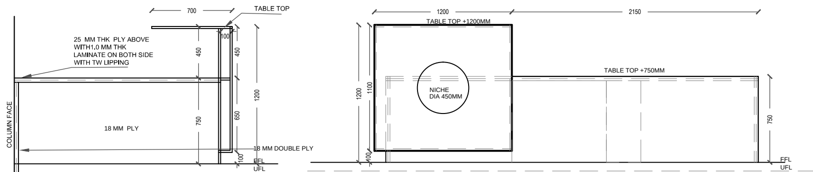
SECTION X-X
