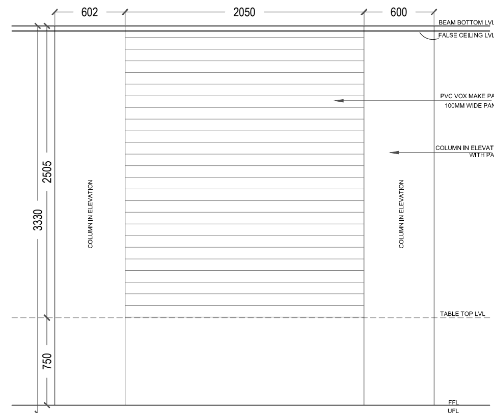
RECEPTION WALL DETAIL ELEVATION 'A'
