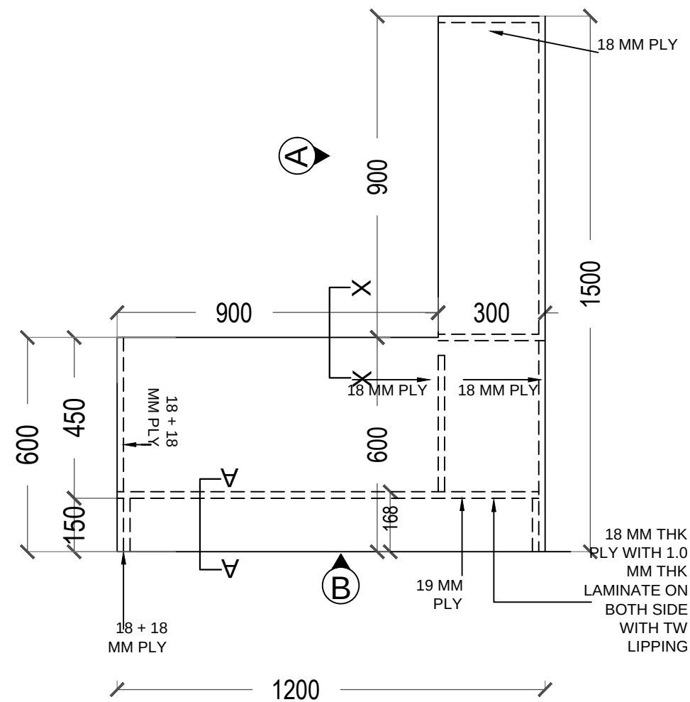
PLAN ABOVE TABLE TOP
