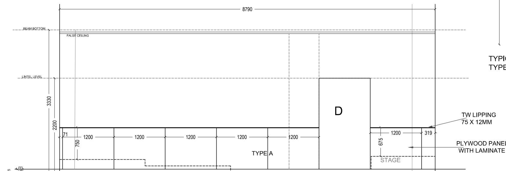
ELEVATION C
