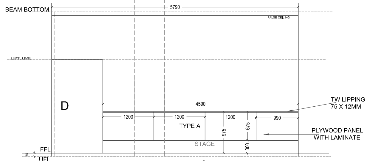
ELEVATION D
