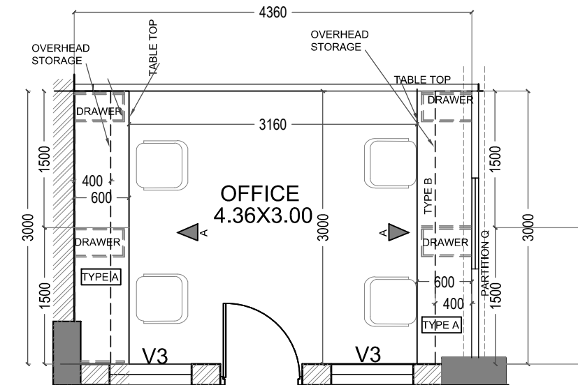
KEY PLAN-OFFICE TABLE 2ND FLOOR
