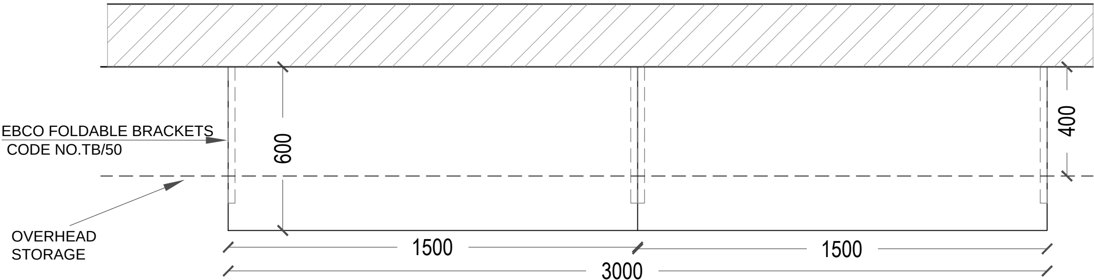
PLAN OF FOLDABLE TABLE
