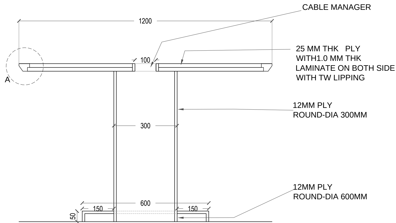
SECTION
