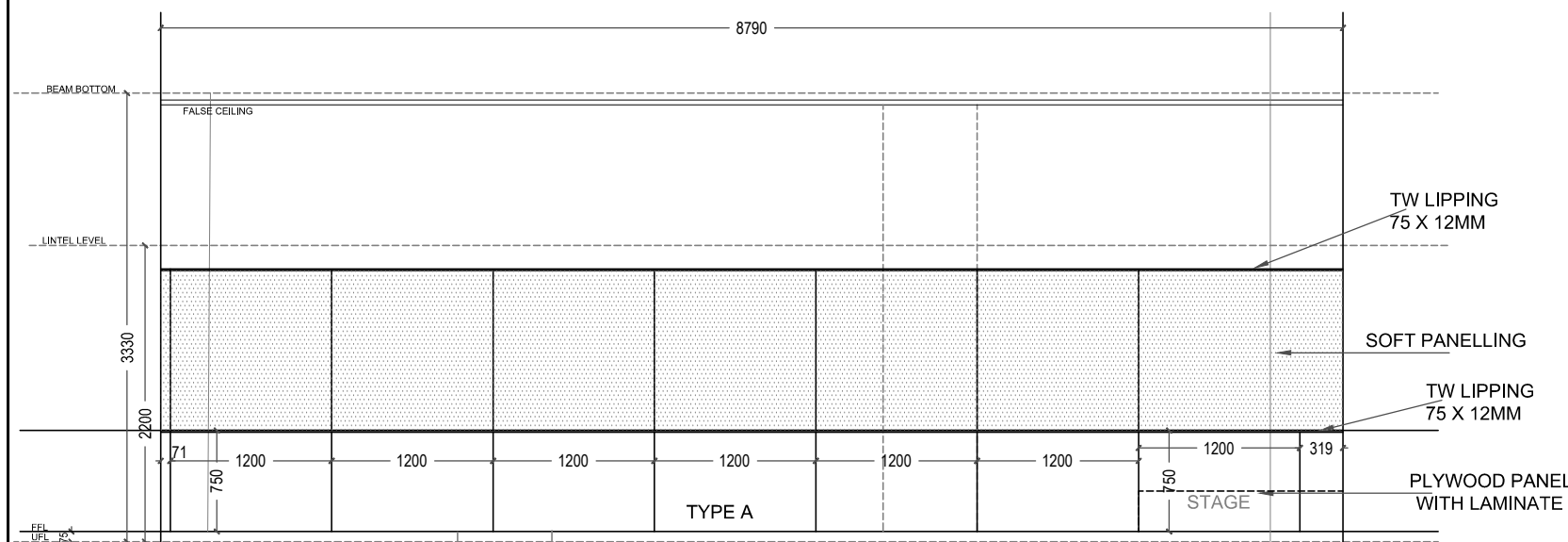
ELEVATION C
