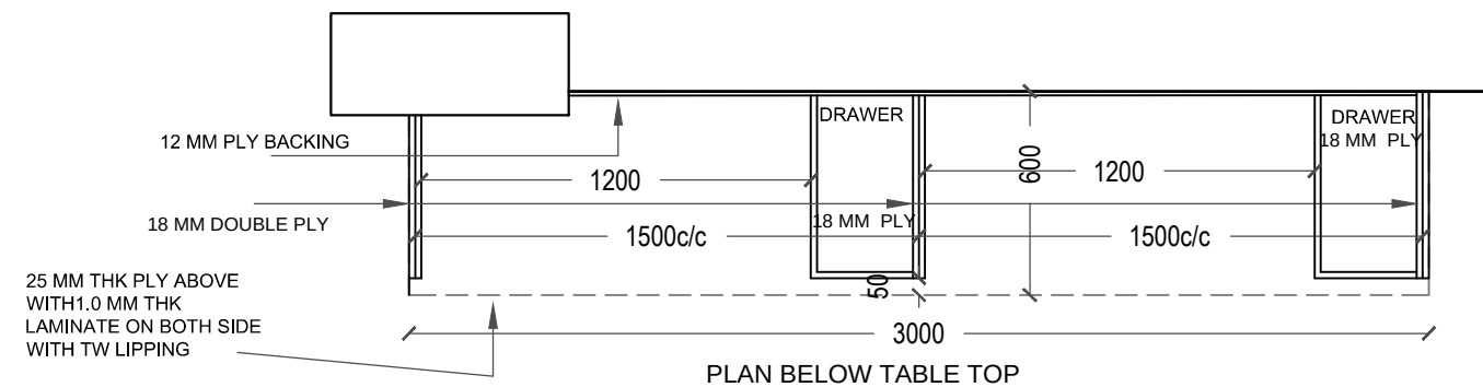
KEY PLAN-OFFICE TABLE 2ND FLOOR
