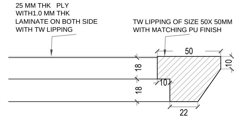
DETAIL AT 'A'
