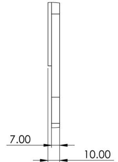
DETAIL B SCALE 1 : 2
