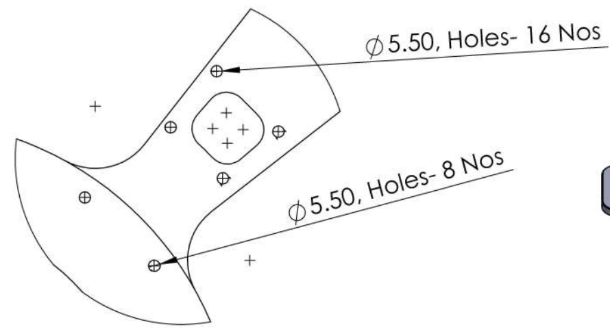
DETAIL D SCALE 2 : 5
