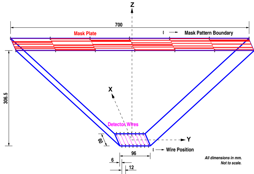
Figure 1. SSM camera.
