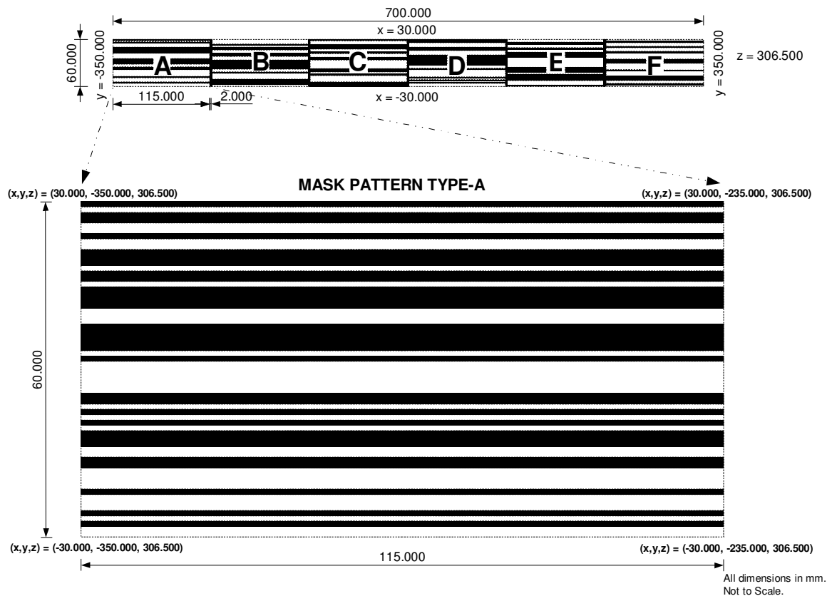
Figure2. Mask Plate
