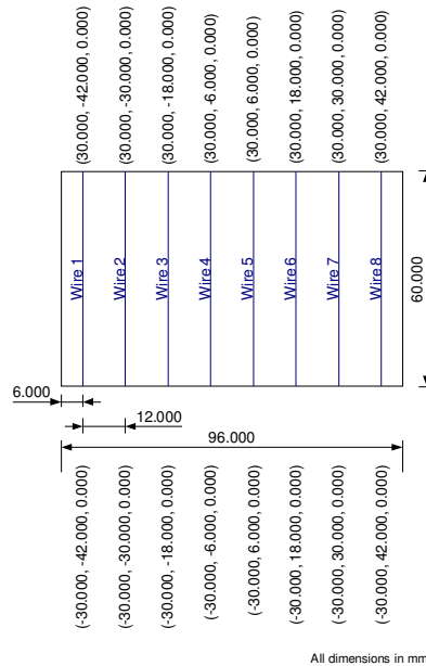
Figure 3. Detector Plane
